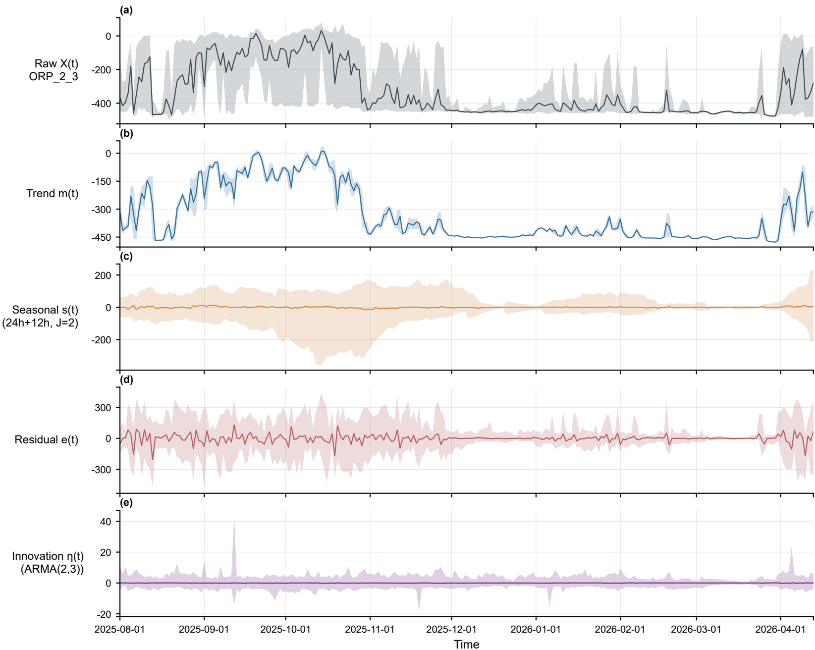
Full-span daily overview — ORP_2_3 (pre_anoxic_rear, min) [2025-08-01~2026-04-13]
